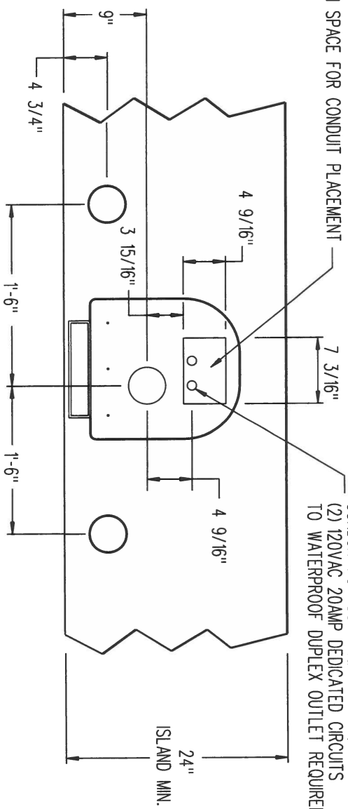
PLAN VIEW
