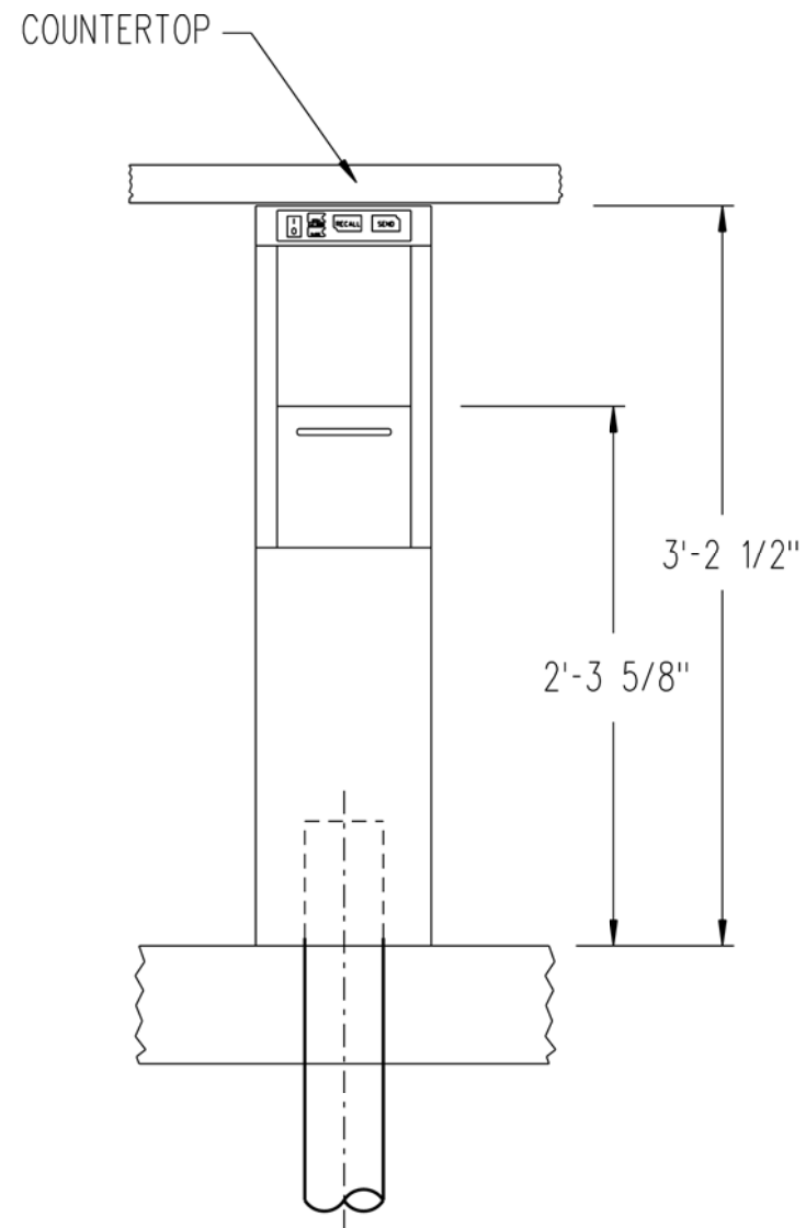
FRONT VIEW
