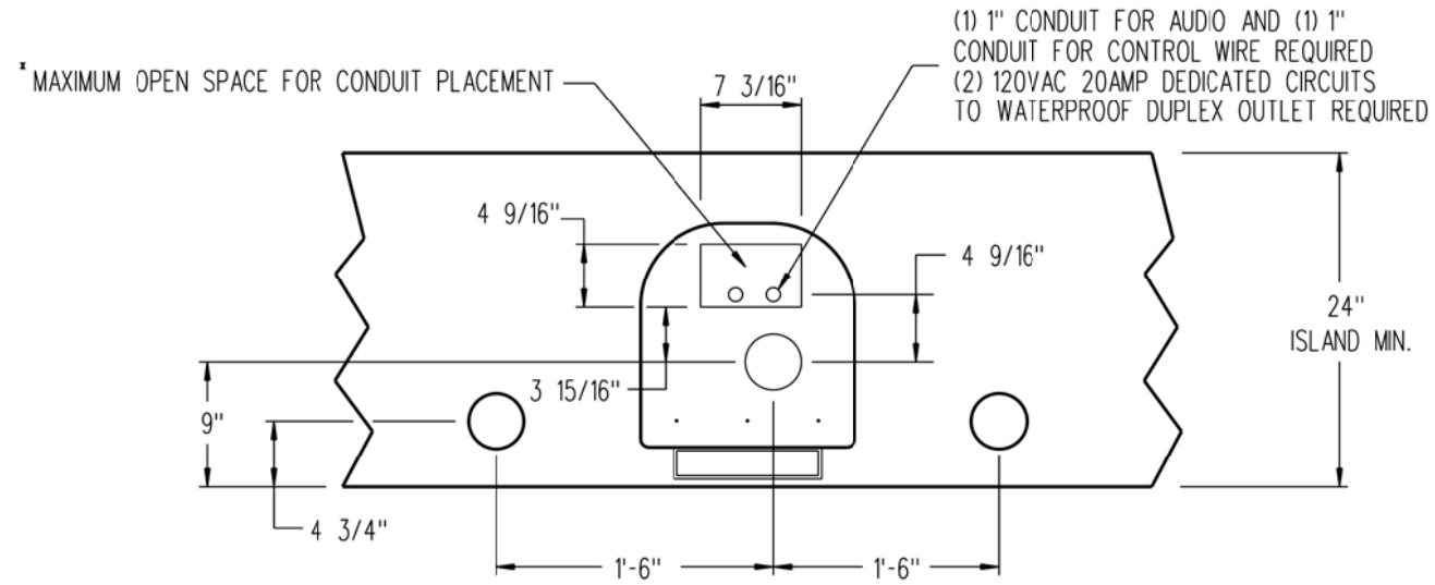
PLAN VIEW
