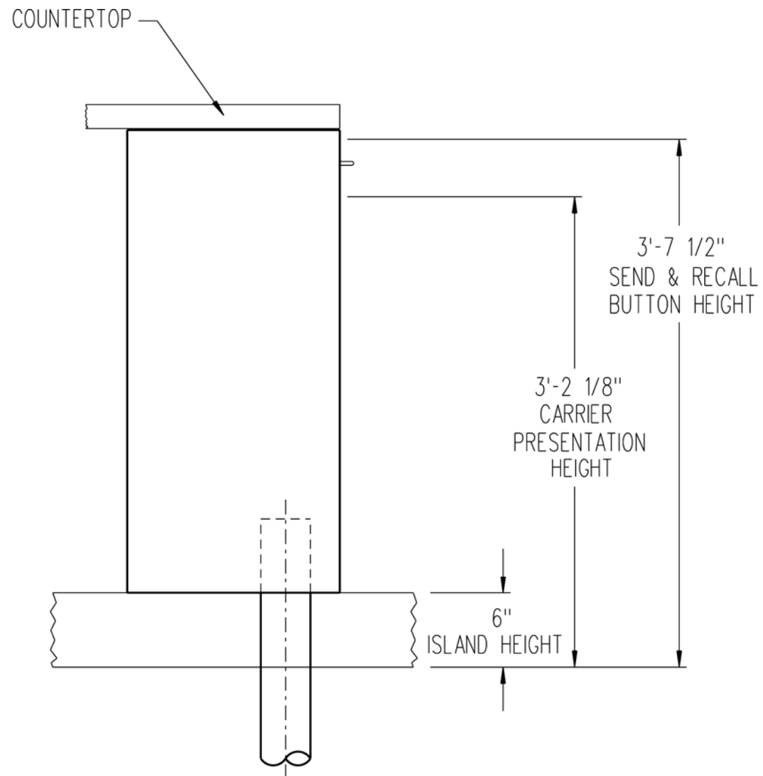
SIDE VIEW
