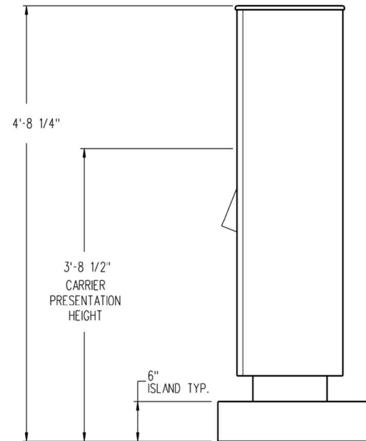
SIDE VIEW
